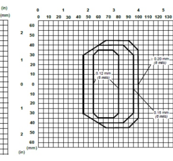
DS2100N-2204 (High Performance HR)
