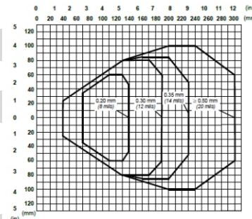
DS2100N-1204 (High Performance SR)
