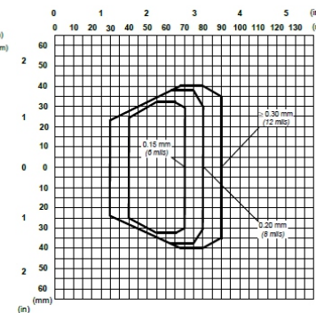
DS2100N-2204 (High Performance HR)
