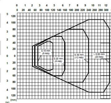
DS2100N-1204 (High Performance SR)
